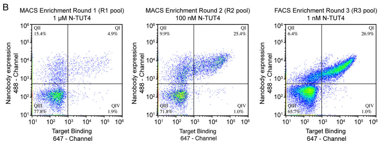
Fig. 2. Discovery of nanobody inhibitors of NTUT 282–759 . (A) Schematic flowchart of nanobody discovery for NTUT 282–759 . (I) MACS enrichment to enrich NTUT 282–759 binders. (II) FACS enrichment to sort high-affinity binders. A schematic of flow cytometry data were drawn to illustrate the sort gate. (III) Inhibitor screening by a functional epitope selection process. (B) Flow cytometry of NTUT 282–759 nanobody binders in two MACS enrichment pools (round 1 pool and round 2 pool) and FACS enrichment (round 3 pool). Nanobodies expressed on the yeast surface were labeled by Alexa Fluor 488 conjugated anti-HA antibodies. Biotinylated NTUT 282–759 was stained with Alexa 647-conjugated streptavidin.
